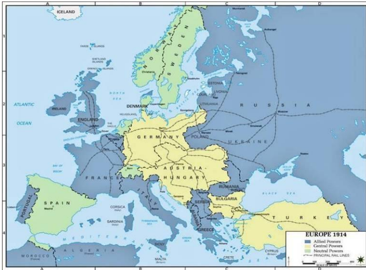
Figure-1: European Political Frontiers in 1914
